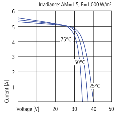
Current-voltage characteristics of PV module LORENTZ LA160-24S at various cell temperatures.
