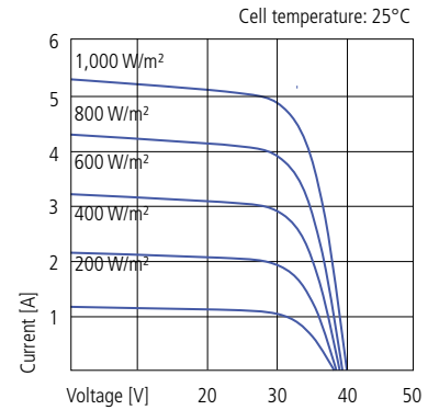
Current-voltage characteristics of PV module LORENTZ LA160-24S at various irradiation levels.
