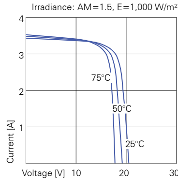
Current-voltage characteristics of PV module LORENTZ LA50-12S at various cell temperatures.
