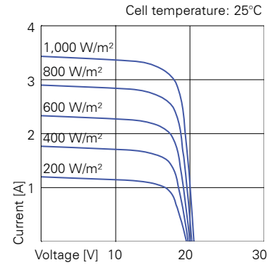
Current-voltage characteristics of PV module LORENTZ LA50-12S at various irradiation levels.
