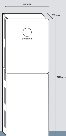
Cabinet option 2 Battery capacity: 5.0-15.0 kWh
